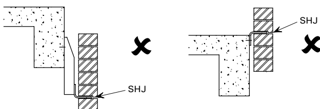
Non-preferred positions of soft horizontal joints in relation to structural beams
